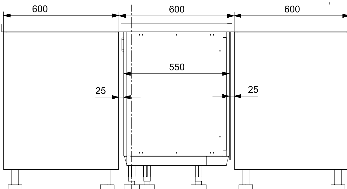
Cross-section frame
