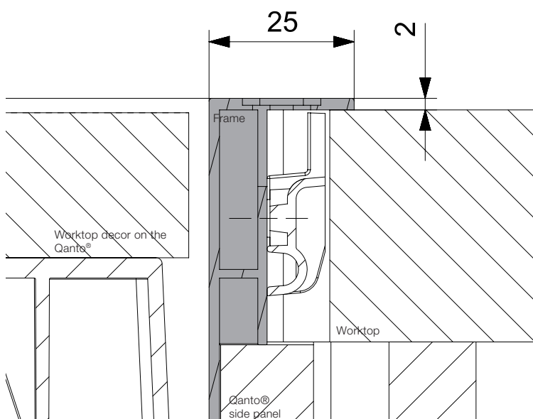
Cross-section frame
