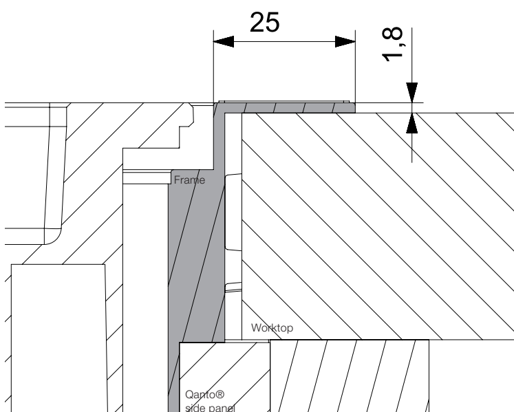
Cross-section frame
